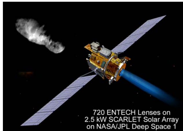
Fig. 5 – SCARLET Array on Deep Space 1
