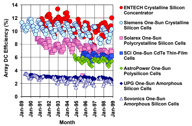
Fig. 4 – PVUSA Long-Term Performance Data
