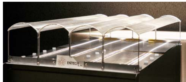
Fig. 6 – Stretched Lens Array (SLA) Prototype
